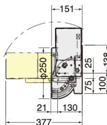
Center height at 90° : 155mm
